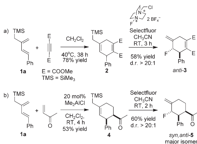
Scheme 2. Sequential cycloaddition–fluorination.
